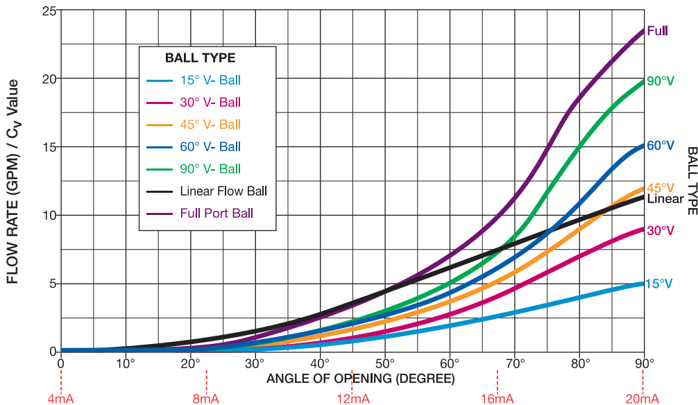
3/4" Valve *
